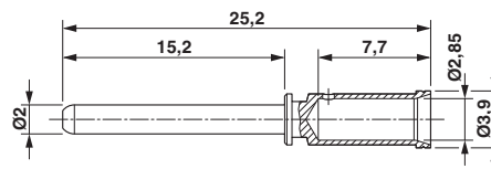
Dimensional drawing
