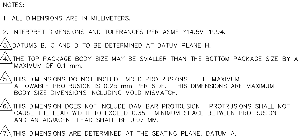
Figure 3. MCF5207CAB166 Package Dimensions (Sheet 2 of 2)
