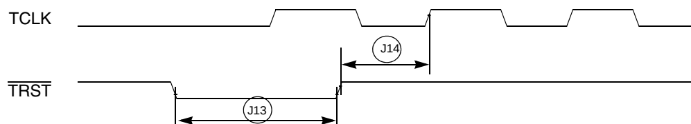
Figure 31. \overline{\text{TRST}} Timing
