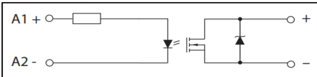
Simplified circuit diagram 2 A, 24 VDC version with MOS-FET Output
