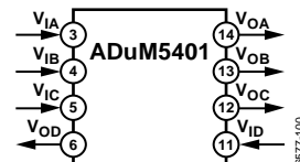
Figure 2. ADuM5401
