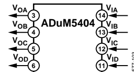
Figure 5. ADuM5404
