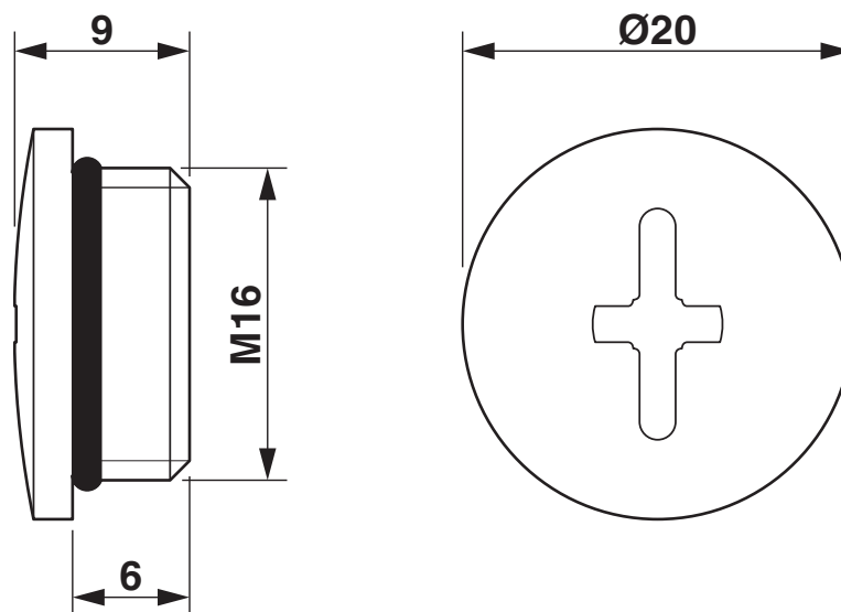
Dimensional drawing
