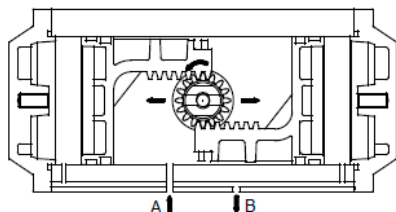
CCW-counter-clockwise
