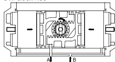
CW-clockwise
