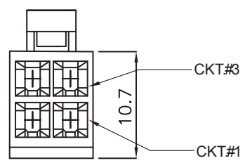
Dimensions for 4pins & 2pins connector
