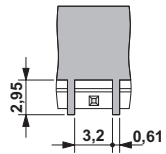
Drilling diagram
