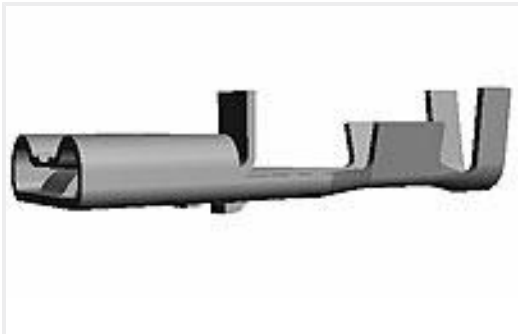
TE Part #170328-1 250 PL MKII REC. 18-14AWG PTBR
