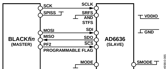
Figure 56. SPI Mode Serial Port Connection to Blackfin DSP
