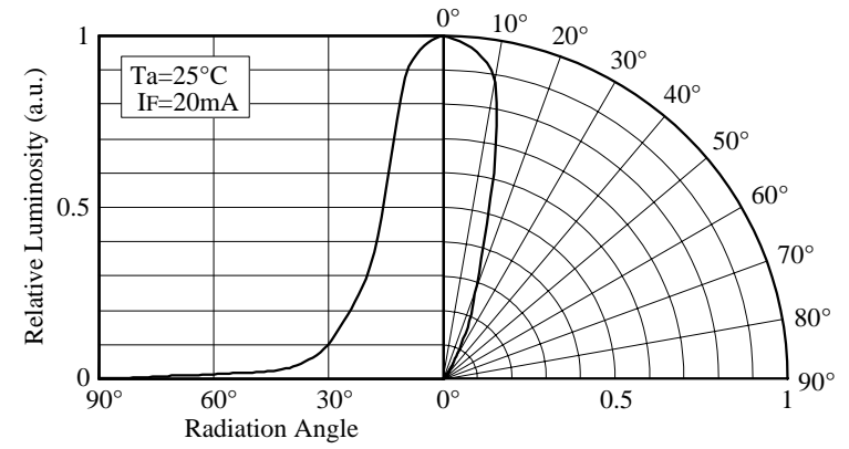
■ Directivity (NSPG510(S))
