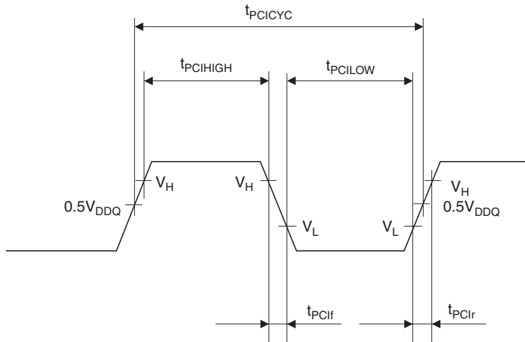
Figure 23.70 PCI Clock Input Timing
