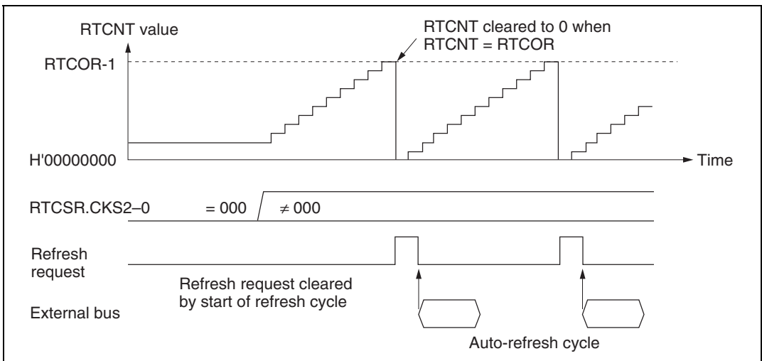
Figure 13.35 Auto-Refresh Operation
