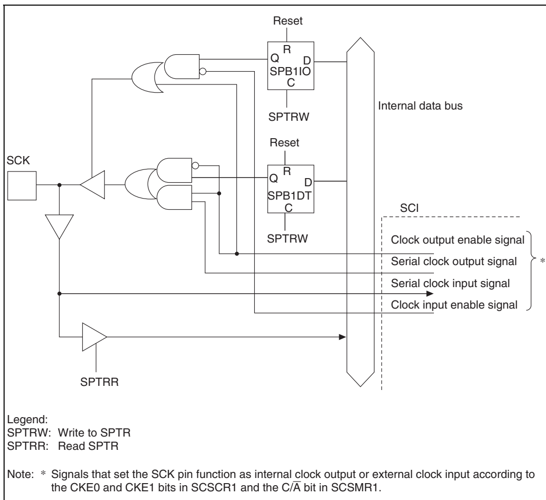
Figure 18.3 SCK Pin
