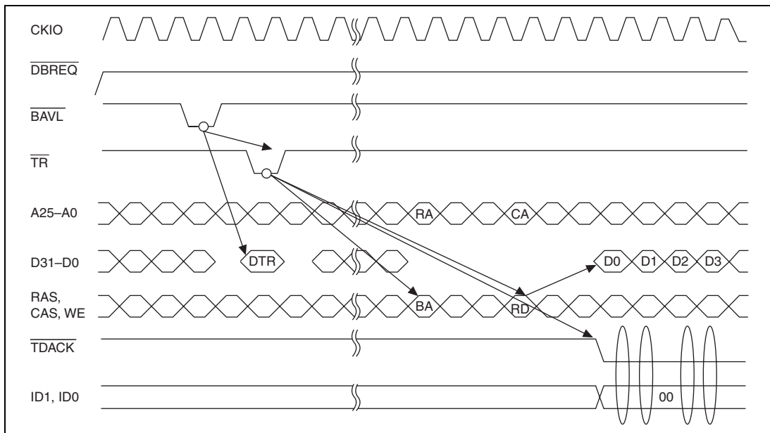
Figure 14.29 Single Address Mode/Burst Mode/External Device → External Device 32-Byte Block Transfer/Channel 0 On-Demand Data Transfer
