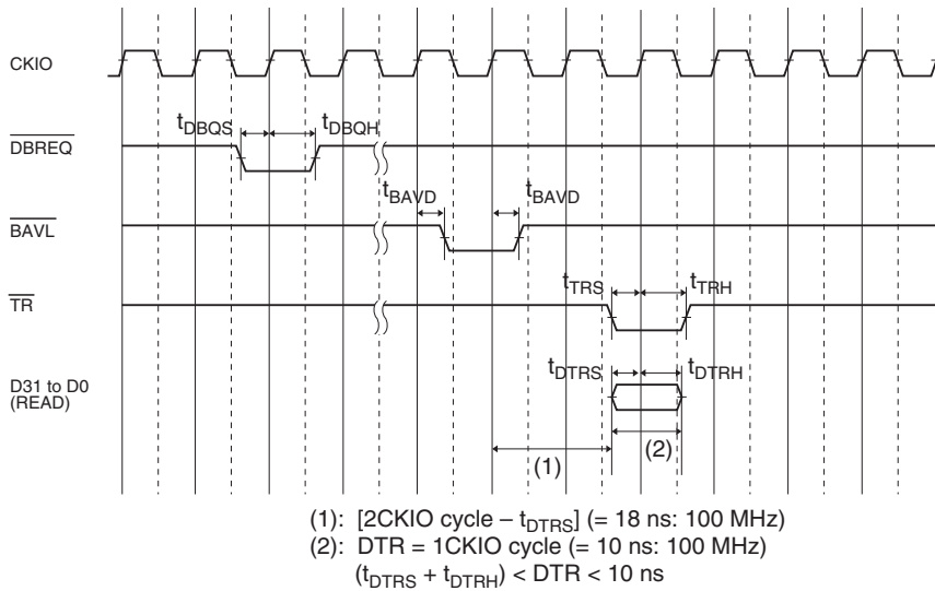
Figure 23.64 (b) \overline{\text{DBREQ}}/\overline{\text{TR}} Input Timing and \overline{\text{BAVL}} Output Timing
