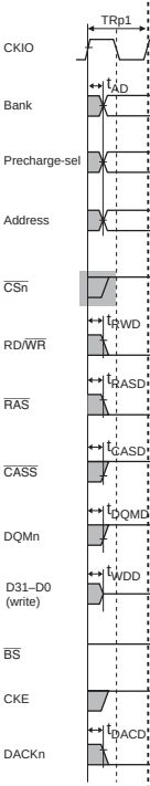
Figure 23.36 DRAM 1038 Title amended Bus Cycle (EDO Mode, RCD [1:0]=00, AnW[2:0]=000, TRC[2:0]=001)
