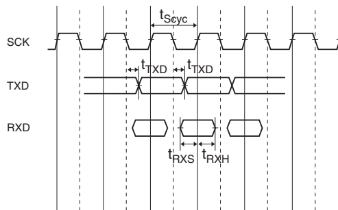
Figure 23.62 SCI I/O Synchronous Mode Clock Timing
