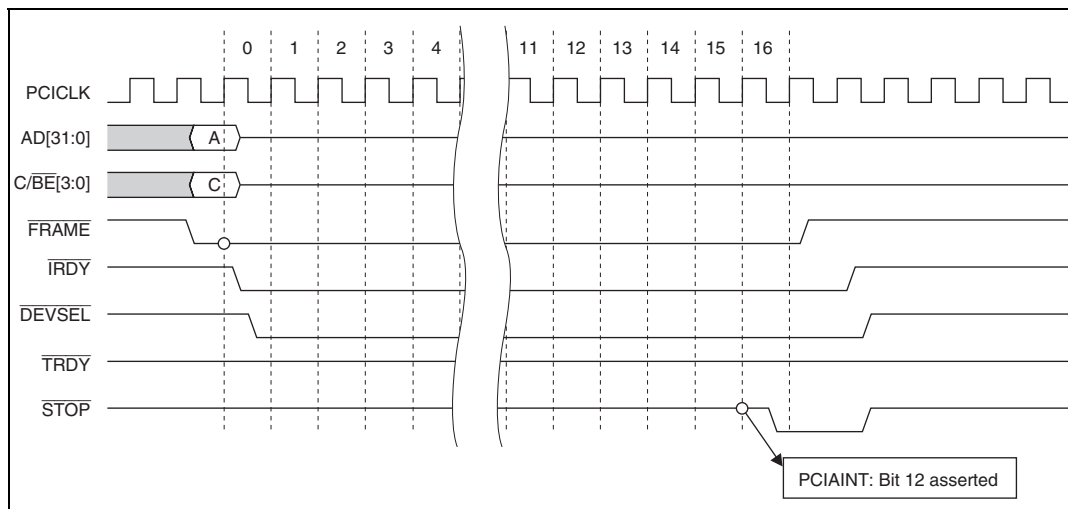
Figure 22.24 Target Bus Timeout Interrupt Generation Example 1 (Example in which the Target Device Asserts STOP at the Sixteenth Clock Cycle after FRAME Was Asserted)
