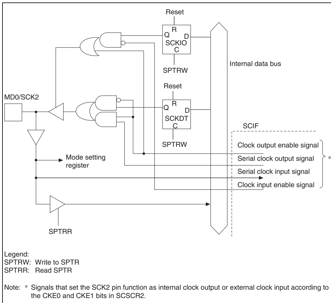
Figure 18.8 MD0/SCK2 Pin
