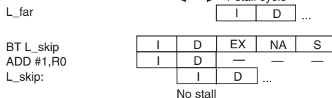
Figure 8.3 Examples of Pipelined Execution
