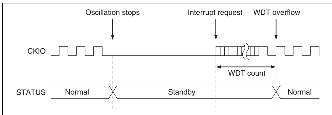
Figure 9.3 STATUS Output in Standby → Interrupt Sequence
