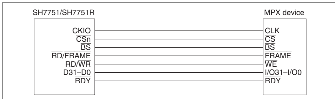
Figure 13.51 Example of 32-Bit Data Width MPX Connection
