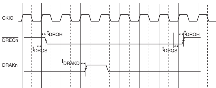
Figure 23.64 (a) \overline{\text{DREQ}} /DRAK Timing
