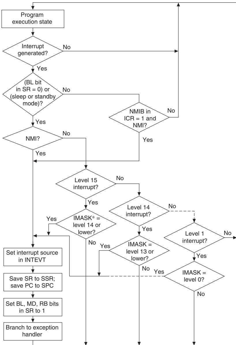
Figure 19.3 Interrupt Operation Flowchart
