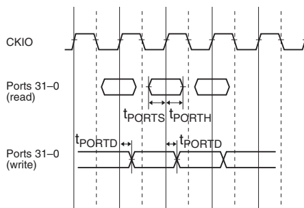
Figure 23.63 I/O Port Input/Output Timing
