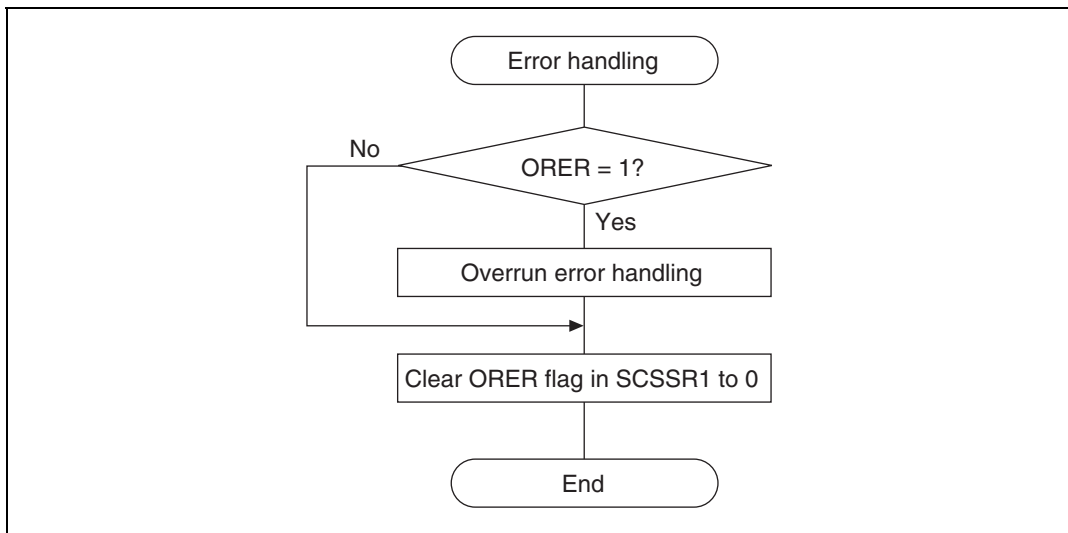
Figure 15.22 Sample Serial Reception Flowchart (2)
