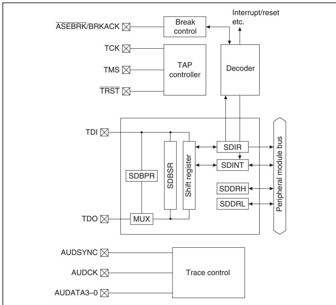
Figure 21.1 Block Diagram of H-UDI Circuit
