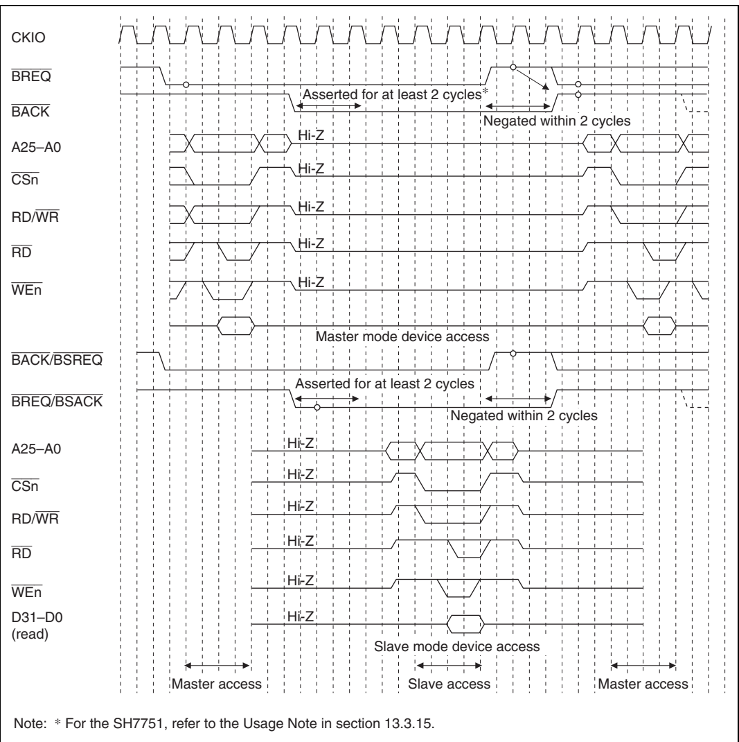
Figure 13.69 Arbitration Sequence
