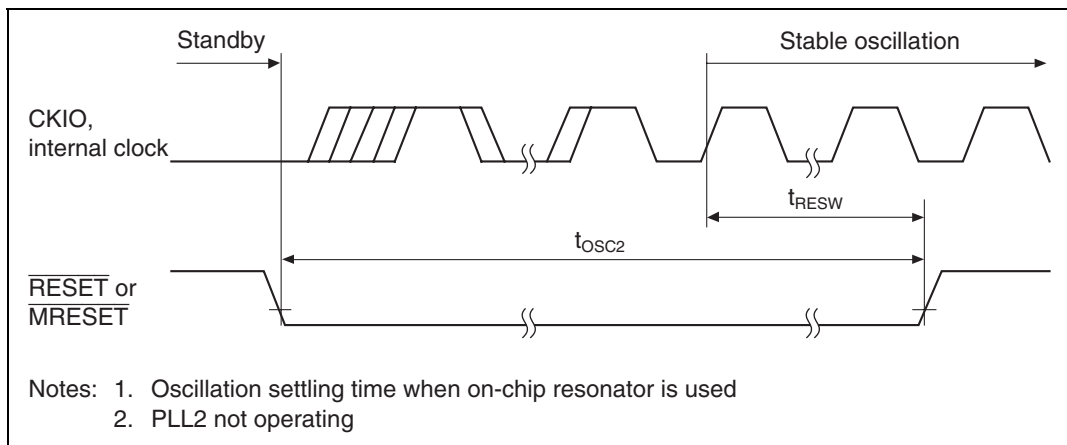
Figure 23.4 Standby Return Oscillation Settling Time (Return by \overline{\text{RESET}} or \overline{\text{MRESET}} )
