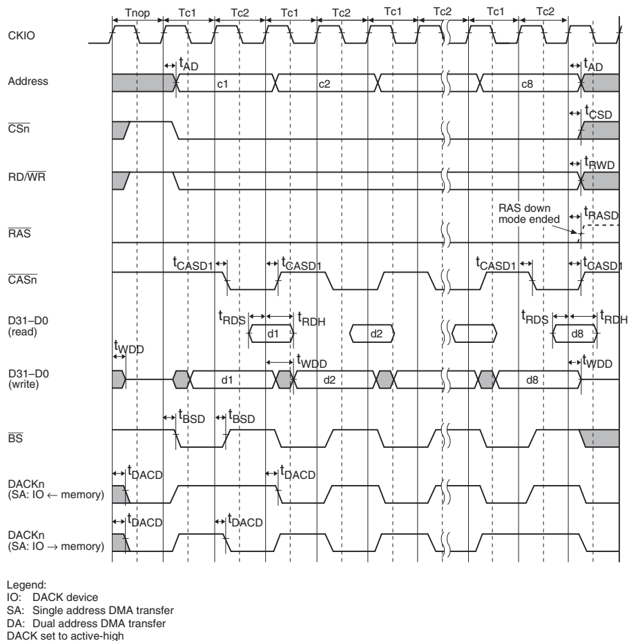
Figure 23.46 DRAM Burst Bus Cycle: RAS Down Mode Continuation (Fast Page Mode, RCD [1:0] = 00, AnW [2:0] = 000)
