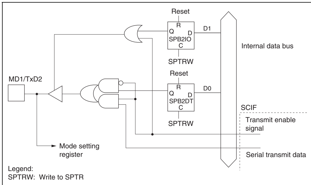
Figure 16.4 MD1/TxD2 Pin
