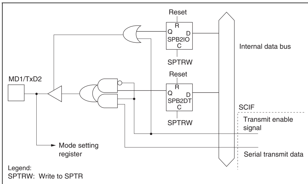
Figure 18.6 MD1/TxD2 Pin
