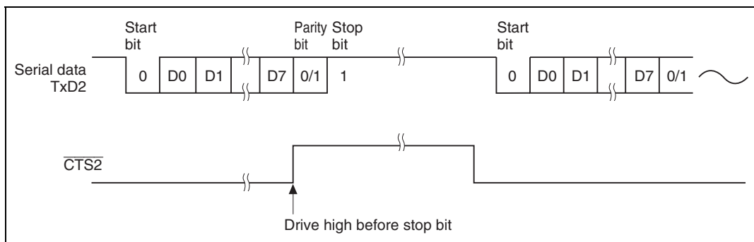
Figure 16.10 Example of Operation Using Modem Control ( \overline{\text{CTS2}} )
