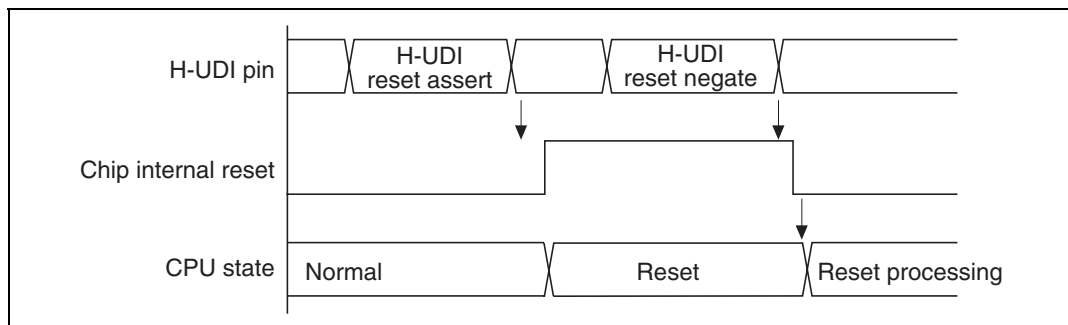
Figure 21.3 H-UDI Reset
