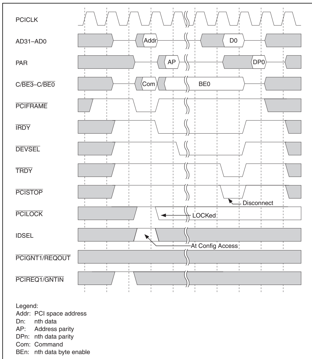
Figure 22.11 Target Read Cycle in Non-Host Mode (Single)
