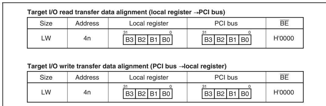
Figure 22.22 Data Alignment at Target I/O Transfer (Both Big Endian and Little Endian)
