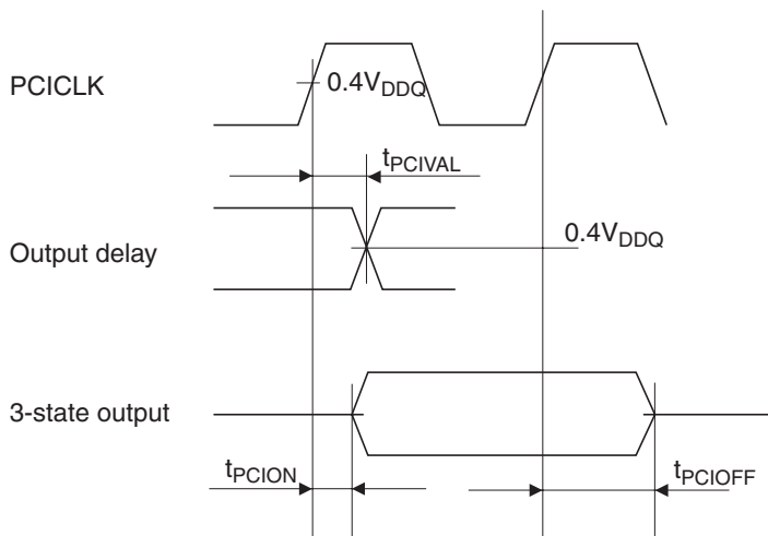
Figure 23.71 Output Signal Timing
