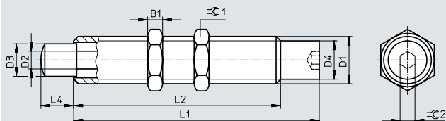
Shock absorber in end position
