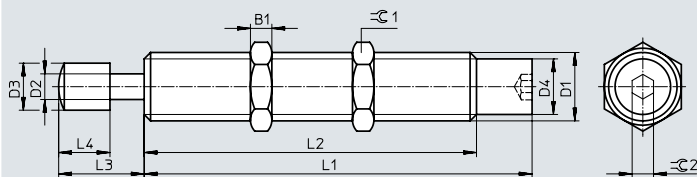
Shock absorber in end position
