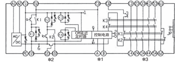
G9SA-TH301 (AC100V~240V)
