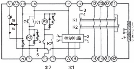
G9SA-501 (AC/DC24V)
