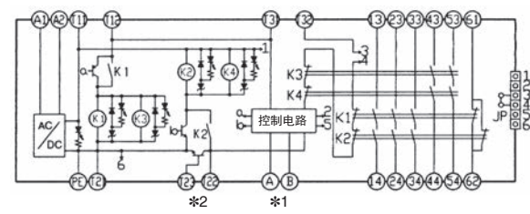
G9SA-321-T□ (AC100V~240V)
