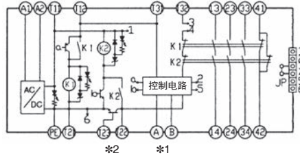
G9SA-501 (AC100V~240V)
